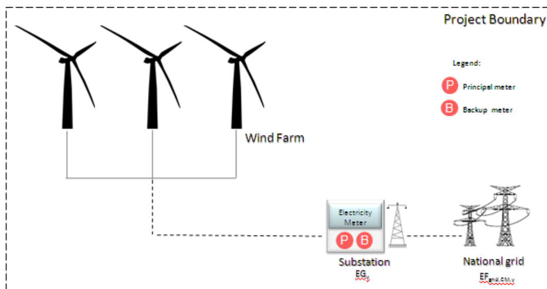
Figure 4 - Project boundary
