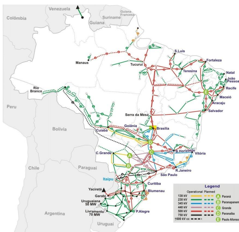
Figure 8 – Brazilian Interconnected System.
