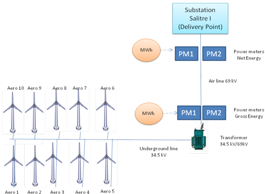
Figure 10. Simplified wiring diagram
