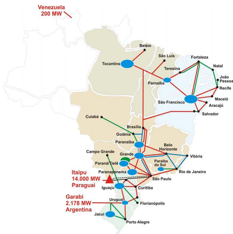
Figure 8. National Interconnected System
