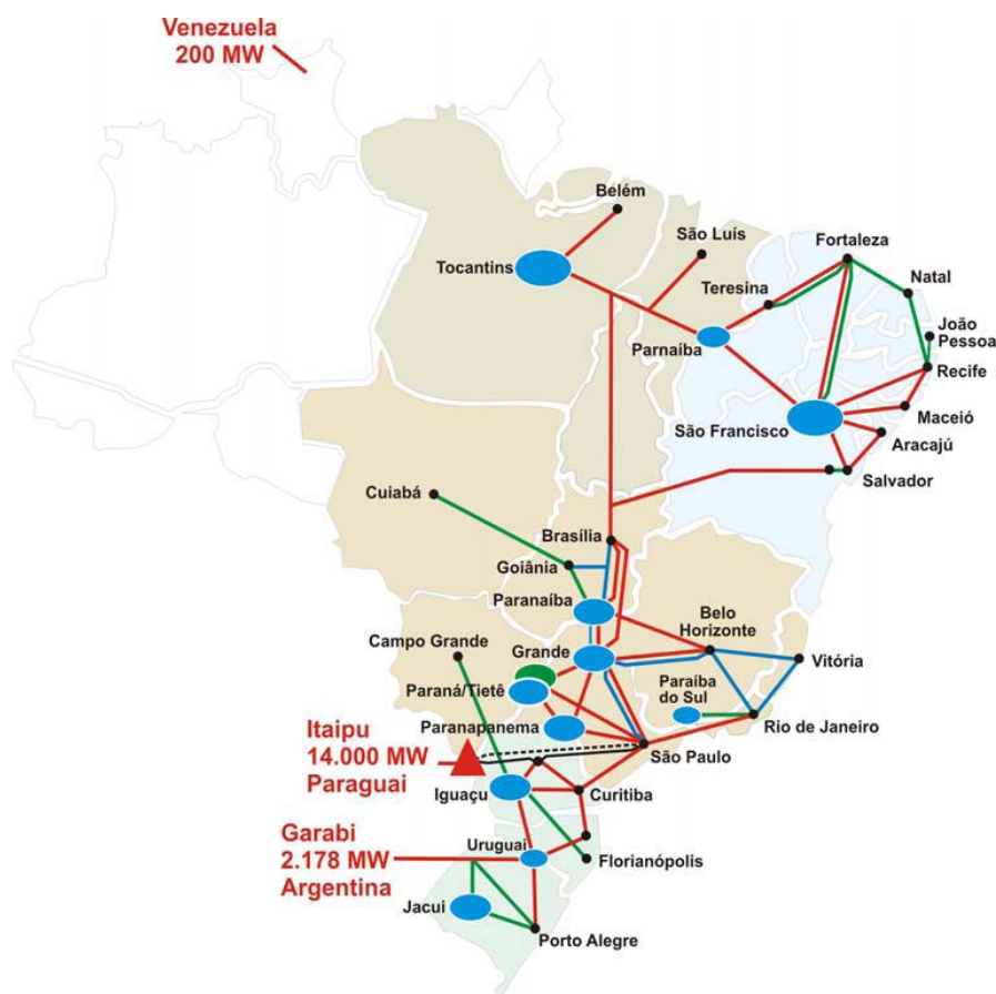
Figure 6. National Interconnected System
