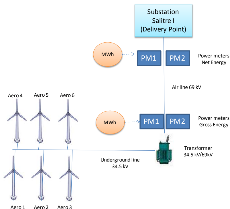
Figure 8. Simplified wiring diagram
