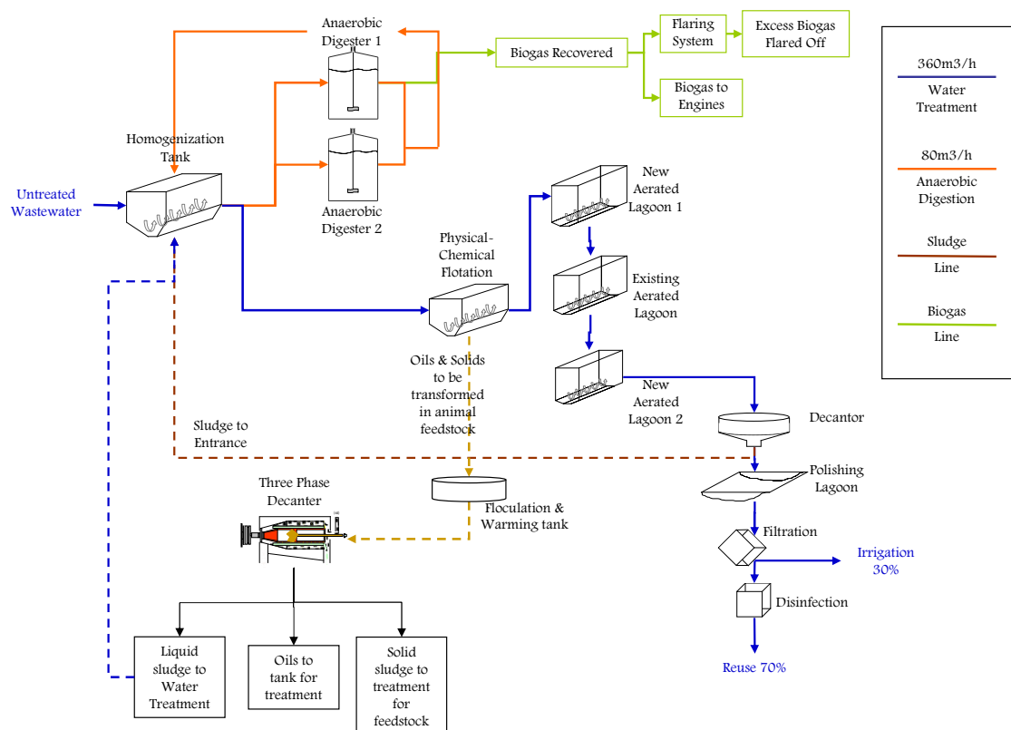
Fig. 5. When production capacity increases, out of the inlet water flow, 80m³/h from the inflow wastewater are conducted to anaerobic digestion. After digestion, this water inflow meets the remaining water flow at the homogenization tank, before entering the physical-chemical flotation tank. After this treatment step, wastewater is conducted to the new & newly equipped aerated serial lagoons, where water flow is treated through organic matter oxidation, thus avoiding the methane generation and the uncontrolled release to the atmosphere. After this new implemented treatment, water is finally discharged at the former facultative lagoon n°2 which is modified onto a secondary decanter. Biogas recovered in the biodigesters is combusted in biogas engines to generate electricity to be consumed by the project equipment or to be exported to the grid. The solid wastes separated by flotation in the PC flotation tank will be dried and treated to be used as animal feedstock. Oils are treated to be reused in other industries. Liquid sludge is redirected to water treatment to maintain the required bacteria level in the homogenization tank to ensure a proper aerated treatment.
