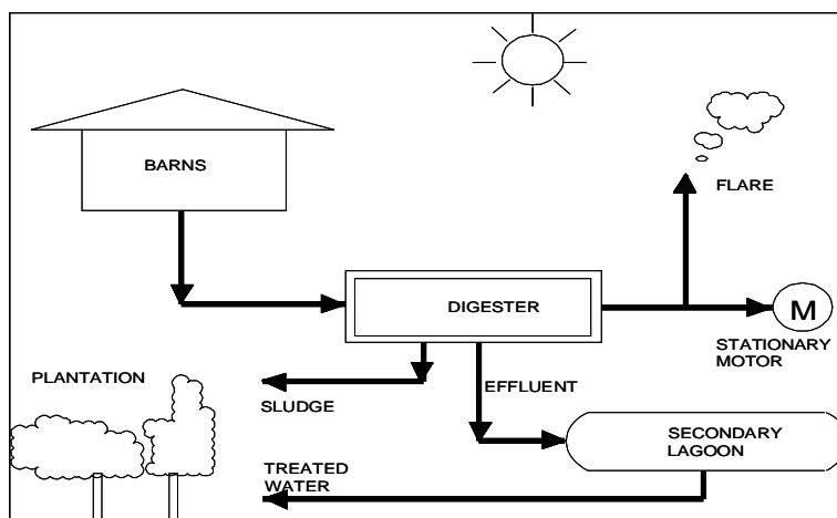
Figure A2. Flowchart of the treatment system
