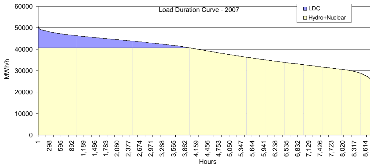
Figure 7 - Load duration curve for the S-SE-CO system, 2007
