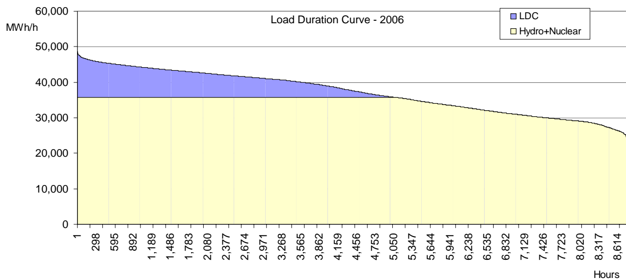
Figure 6 - Load duration curve for the S-SE-CO system, 2006
