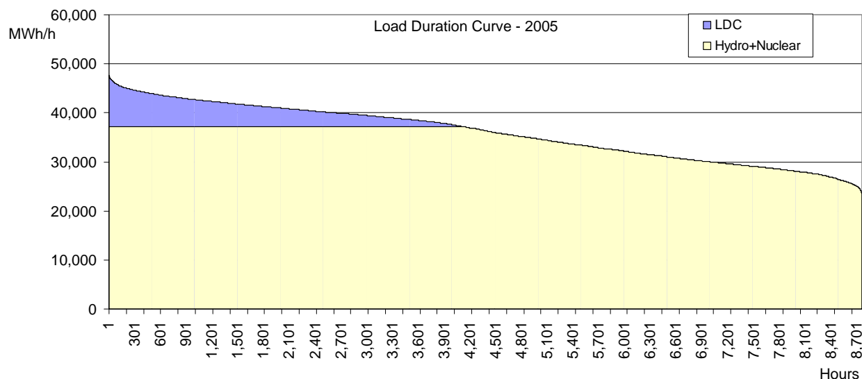
Figure 5 - Load duration curve for the S-SE-CO system, 2005
