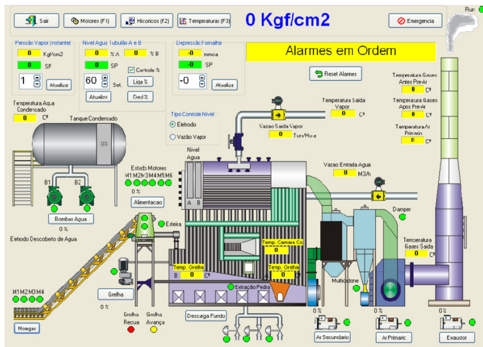
Figure 7 – Control Monitor
