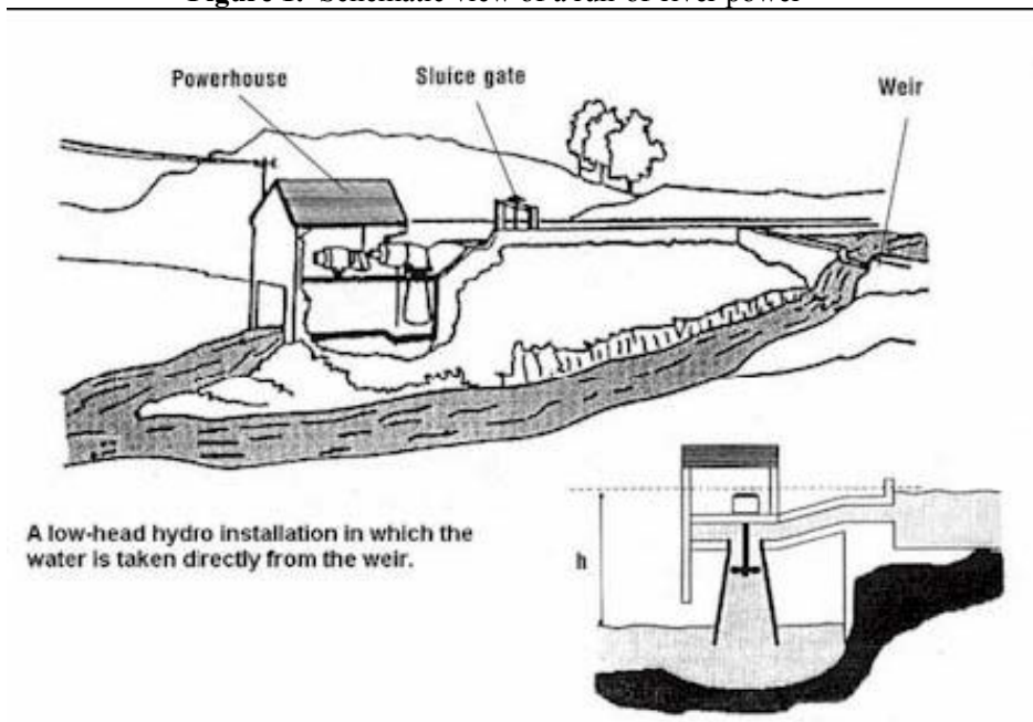
Figure 1. Schematic view of a run-of-river power
