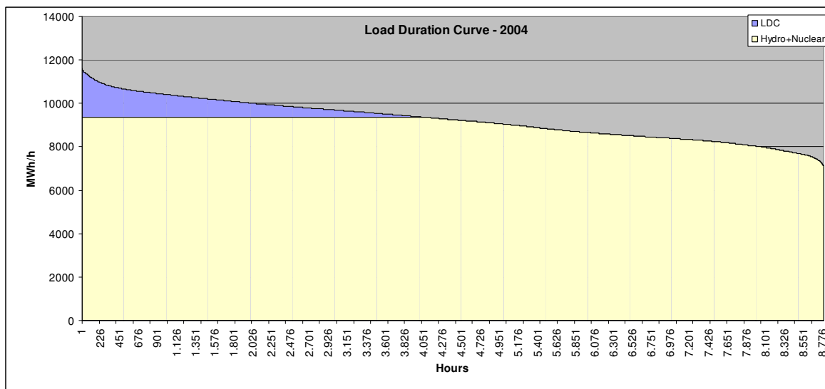
Figure 3.3. Load duration curve for the N-NE system, 2004
