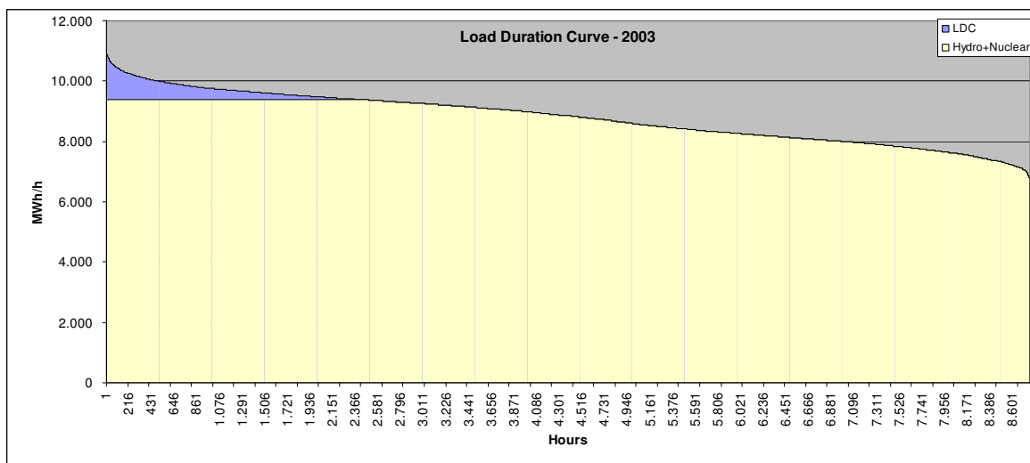
Figure 3.2. Load duration curve for the N-NE system, 2003
