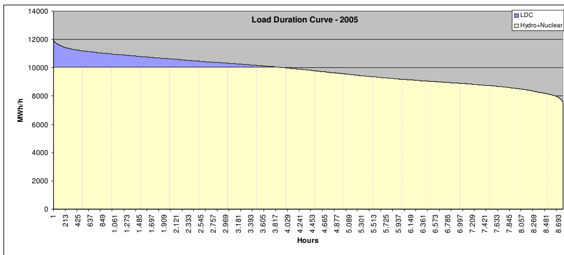
Figure 3.4. Load duration curve for the N-NE system, 2005
