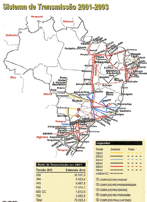
Figure 13 - Brazilian Interconnected System (Source: ONS)
