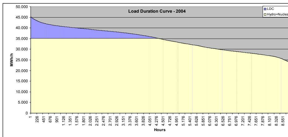
Figure 16 – Load duration curve for the S-SE-CO system, 2004
