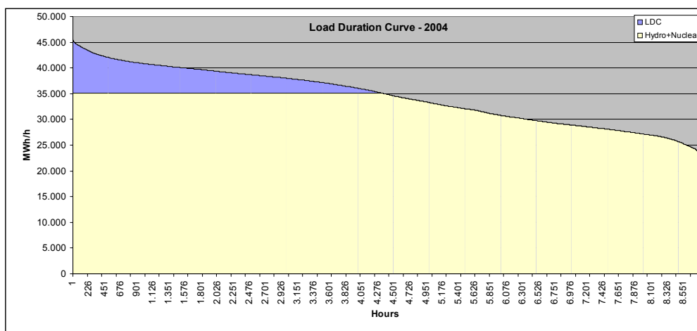
Figure 17 – Load duration curve for the S-SE-CO system, 2004
