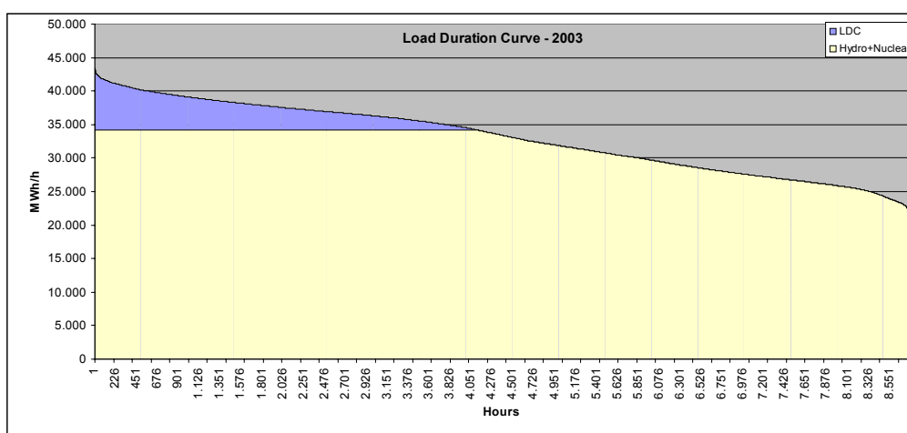
Figure 12 - Load duration curve for the S-SE-CO system, 2003
