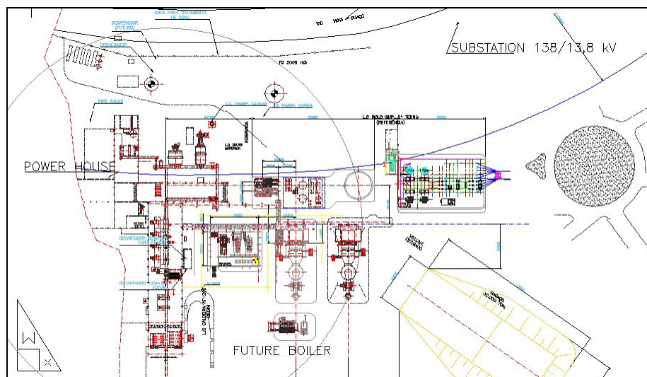
Figure 3: Cresciumal site lay-out and equipment location
