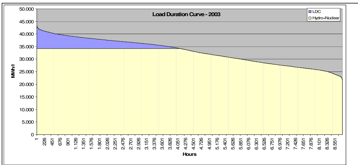
Figure 4: Load duration curve for the S-SE-MW system, 2003
