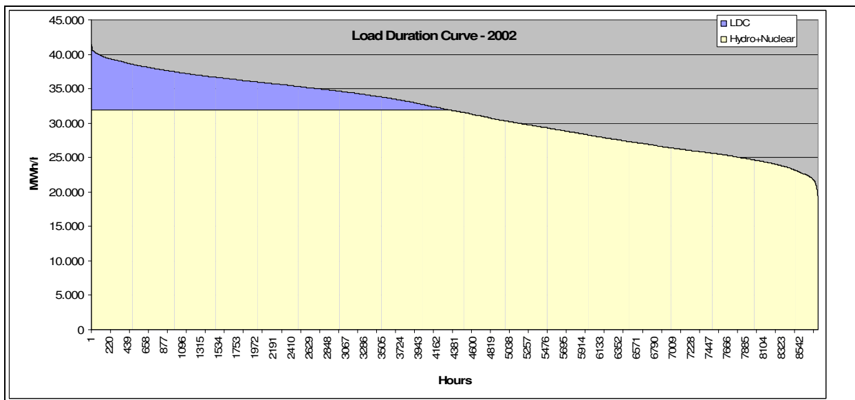
Figure 3: Load duration curve for the S-SE-MW system, 2002
