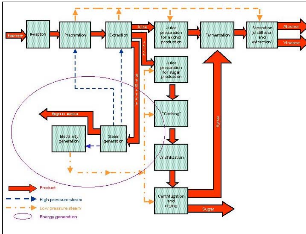
Figure 2 - Flowchart of the electricity generation inside a Sugar and Alcohol Production (Source: Codistil)
