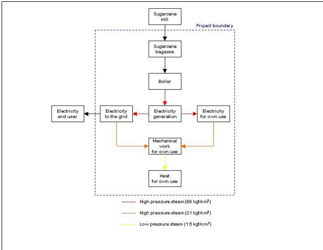
Figure 16 – Flowchart of the Project Boundaries
