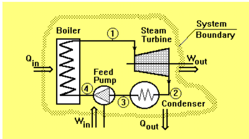
Figure 4 - Rankine Cycle (Source: Taftan Data, 1998)
