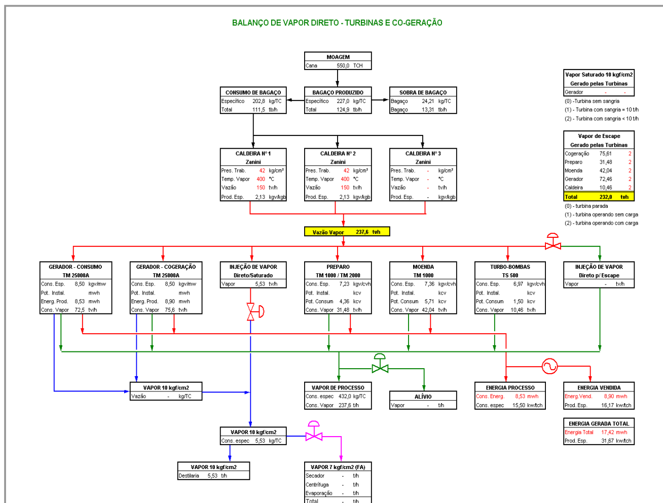
Figure 3: Alta Mogiana's Energy Balance Diagram
