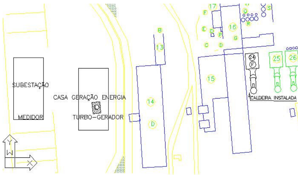
Figure 3. Location of installed equipments for bagasse cogeneration at Cerradinho site - Lay out
