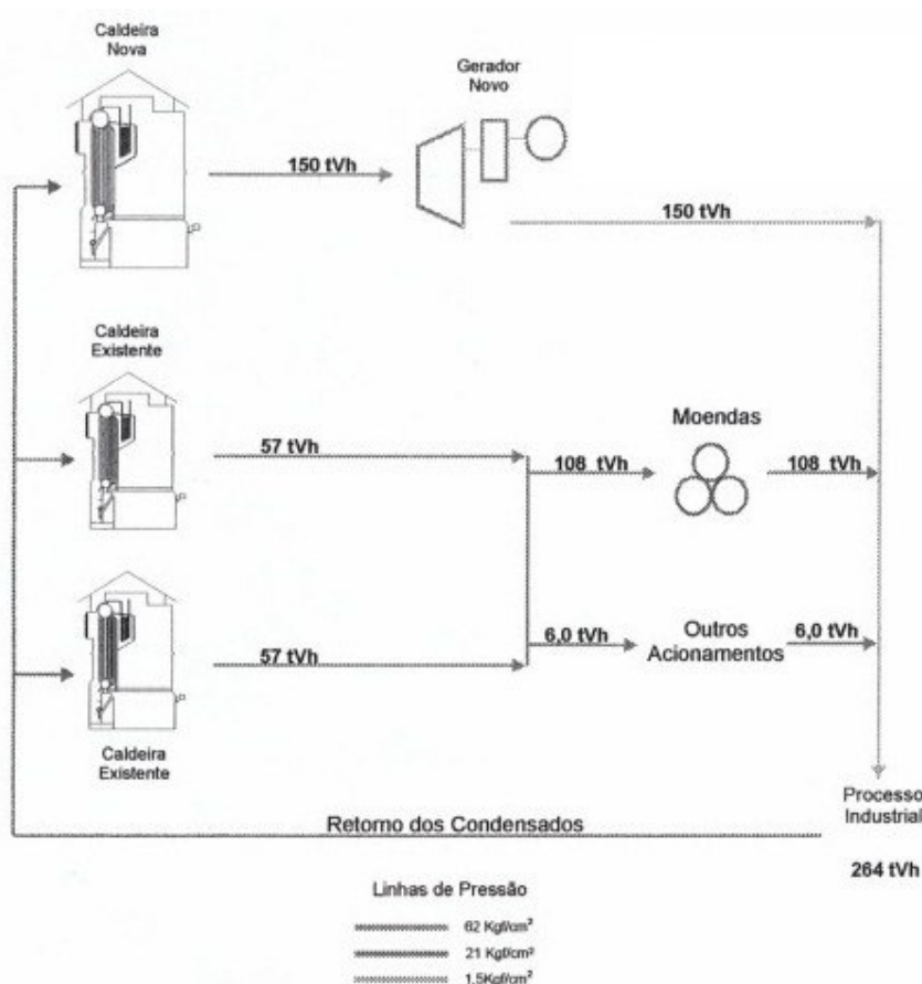
Figure 4. Energy Balance Diagram for Phase 1
