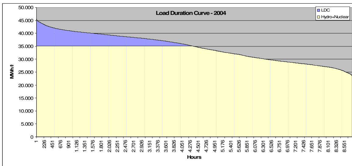
Figure 7. Load duration curve for the S-SE-MW system, 2004
