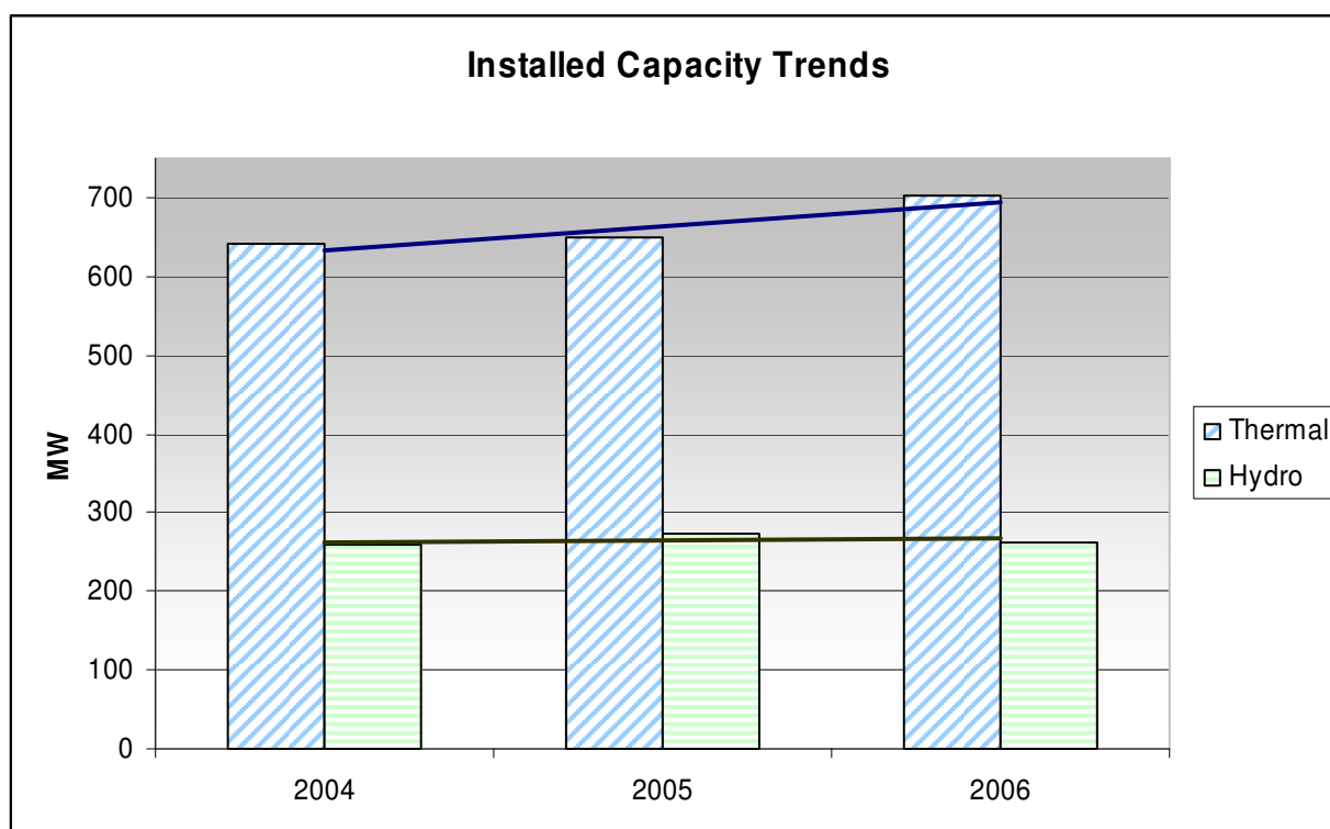
Figure 1 - Installed capacity trends in Rondônia (Souces: Eletrobrás – own elaboration)
