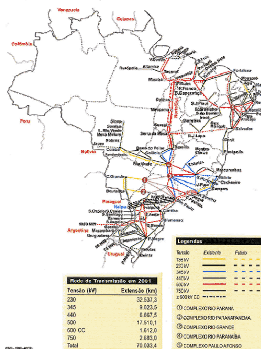
Figure 5 – Brazilian Interconnected System (ONS)
