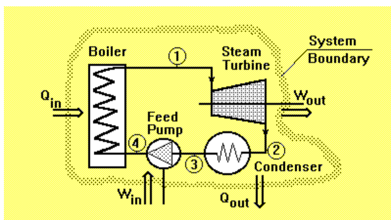
Figure 3 - Rankine Cycle
