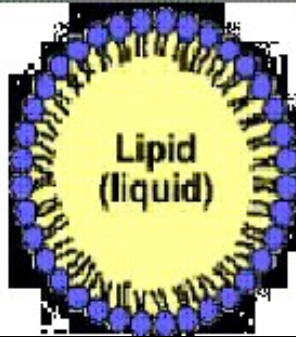
1b Nanoemulsion: Lipid monolayer enclosing a liquid lipid core
