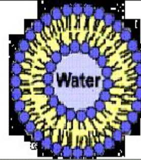
1a Liposome: Lipid bilayer enclosing an aqueous core
