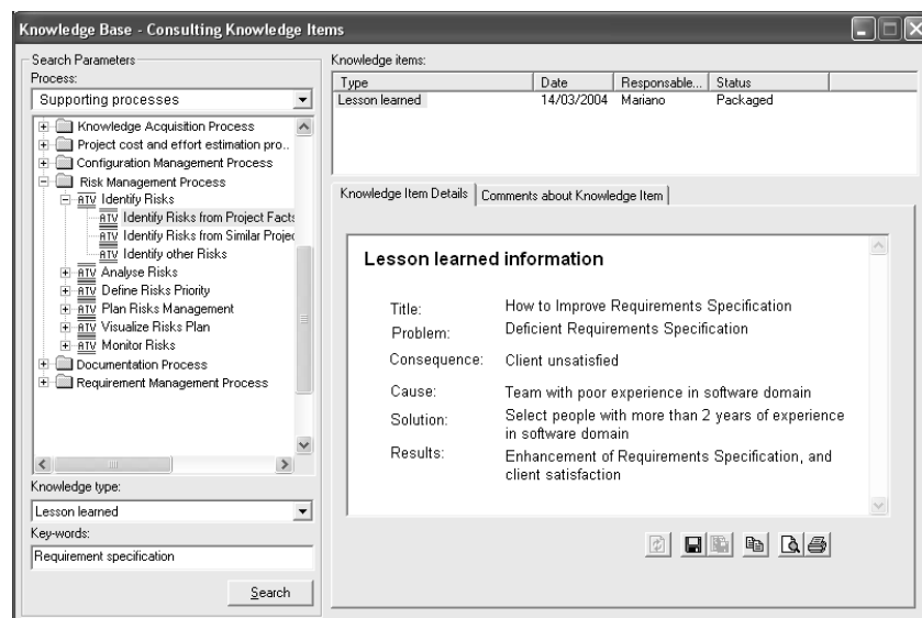
Fig. 4. Acknowledge tool to support search and access to knowledge items related to activity execution.
